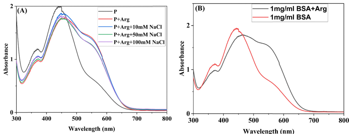
Fig. 3 (A) UV-Vis absorption spectra of P1 (100 μM in the presence of different concentrations of salt (NaCl, 10 to 100 mM)). (B) The UV-Vis absorption spectra of probe P1 and P1 + arginine in the presence of bovine serum albumin (BSA, 1 mg mL -1 ) [red and black lines, respectively].
