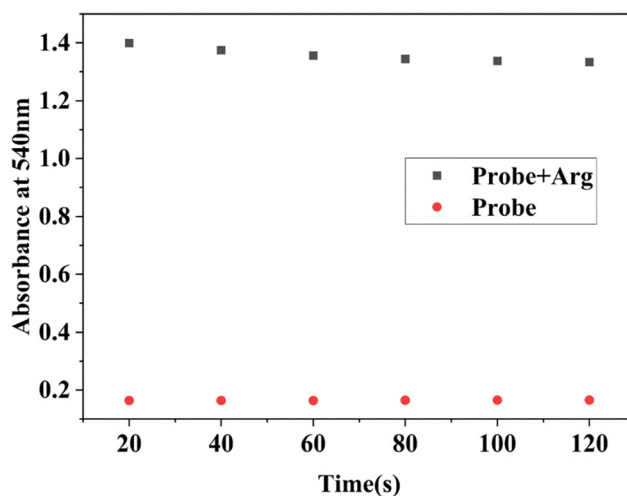
Fig. 4 Time-dependent absorbance at 540 nm of 100 μM probe P1 with 1 equiv. arginine.
