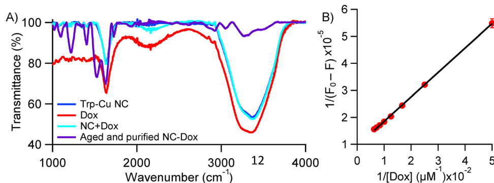
Fig. 4 (A) FTIR spectra of Trp-Cu NC (blue), free Dox (red), Trp-Cu NC + 160 \mu\text{M} Dox before aging (cyan) and aged and purified Trp-Cu NC-Dox nanoconjugate (violet). (B) Benesi-Hildebrand plot to determine the binding constant.
