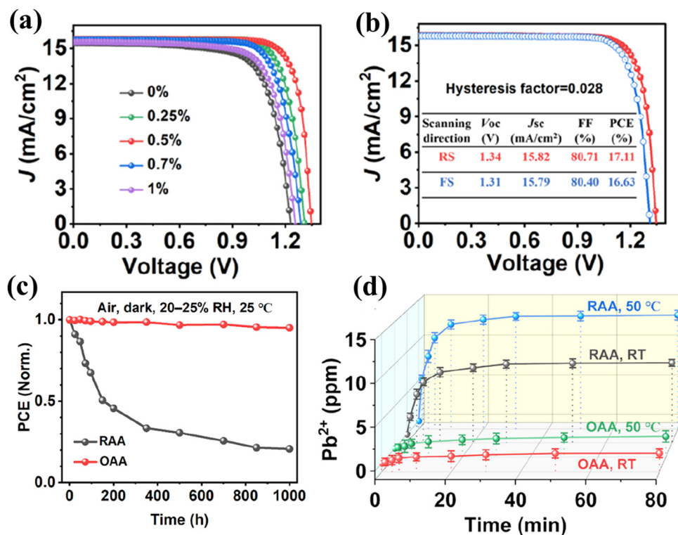
Fig. 12 (a) J-V characteristics of PSCs with different concentrations of BP-9 additives. (b) J-V hysteresis. (c) Stability test at 25 °C in ambient air with 20–25% RH with BP-9(OAA) and pristine device (RAA). (d) Pb 2+ leakage test into deionized water at room temperature and 50 °C of the additive-induced device and pristine device. Reproduced with permission from ref. 206.
