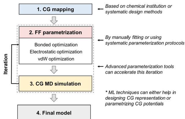
Fig. 2 The workflow for proposing a new IL CG model.
