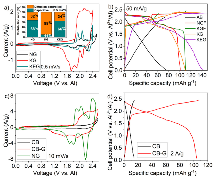
Fig. 7 (a) CV curves of cells with natural graphite (NG), 59 Kish graphite (KG) 61 and kish-based expanded graphite (KEG) 17 cathode and \text{AlCl}_3/\text{[EMIM]Cl} (1.3:1) electrolyte, at a scan rate of 0.5 \text{mV s}^{-1} . Insert is the contribution ratio of these three graphite cathodes. (b) Charging and discharging profiles of cells with various graphitic materials and \text{AlCl}_3/\text{[EMIM]Cl} (1.3:1) electrolyte at 50 \text{mA g}^{-1} . These graphite materials are KG 61 and KEG, 17 and kish graphite flakes (KGF, 2 mm), natural large graphite flakes (NGF, 1 mm) and acetylene black (AB, 26 \mu\text{m} ). 19 (c) CV curves at a scan rate of 10 \text{mV s}^{-1} and (d) charging/discharging profiles at a current density of 2 \text{A g}^{-1} of cells with NG 59 (only used in CV), CB (XC-72) and CB-G (carbon black-derived nanosheet-bricked porous graphite, NSPG-120) 66 cathode and \text{AlCl}_3/\text{[EMIM]Cl} (1.3:1) electrolyte. Adapted with permission from Elsevier. 17 Copyright 2024. Adapted with permission from author. 19 Copyright 2017. Adapted with permission from Springer Nature. 59 Copyright 2024. Adapted with permission from Elsevier. 61 Copyright 2023. Adapted with permission from author. 66 Copyright 2018.
