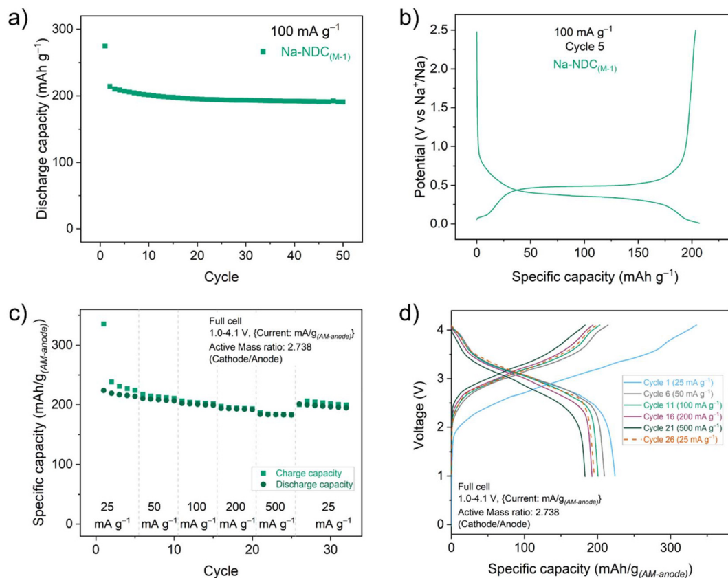
Fig. 2 (a) Discharge capacity and (b) galvanostatic charge/discharge curves for Na-NDC materials (5th cycle) cycled between 0.01–2.5 V at a current rate of 100 mA g -1 . Rate performance for full-cell prepared using Na-NDC (M-1) as anode, (c) discharge capacity at different current rates, cycled five times at every step, and (d) corresponding charge/discharge curves for first cycle of every step.
