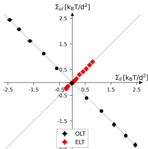
Fig. 3 Leaflet tension space for planar bilayers that contain a total number of N_{II} + N_{UI} = 1682 lipids. 18 The two coordinates are the leaflet tensions \Sigma_{II} and \Sigma_{UI} in the lower and upper leaflets. Negative and positive leaflet tensions describe compressed and stretched leaflets. The reference state with tensionless leaflets, corresponding to \Sigma_{II} = \Sigma_{UI} = 0 , is obtained for the symmetric bilayer with N_{II} = N_{UI} = 841 lipids. The red data points describe elastic deformations with equal leaflet tensions (ELTs), \Sigma_{II} = \Sigma_{UI} . The black data points represent bilayers with opposite leaflet tensions (OLTs), \Sigma_{II} = -\Sigma_{UI} and \Sigma = 0 . All OLT states can be obtained from the reference state by reshuffling lipids from one leaflet to the other and adjusting the base area of the simulation box to obtain tensionless bilayers.
