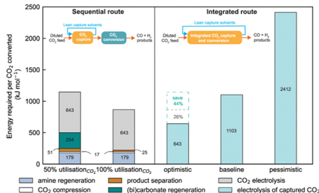
Fig. 23 Energy comparison between the sequential route (conventional CO 2 RR) vs. the integrated route (the c-CO 2 RR route). 33 The optimistic scenario assumes that c-CO 2 RR performs at the same efficiency as the current state-of-the-art CO 2 electrolyzers with a 90% F.E. CO at cell potential of 3 V, the baseline scenario uses Lee et al. 's report of 72% F.E. CO at -0.8 V vs. RHE, 28 and the pessimistic scenario assumes a 40% F.E. CO at a large cell potential of 5 V. Reproduced with permission from ref. 33, copyright 2022 Nature.
