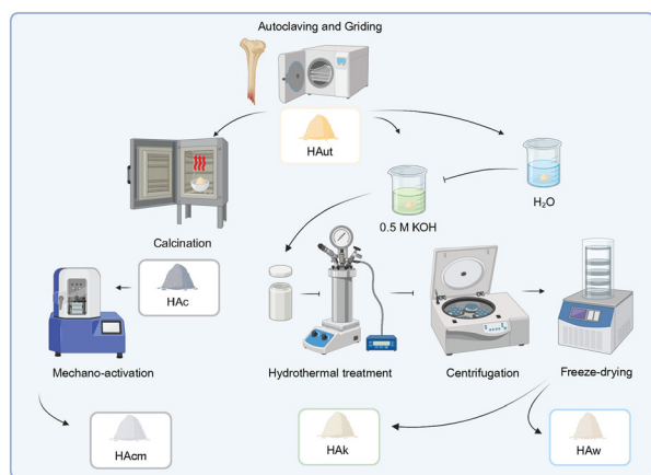
Fig. 1 Flowchart illustrating bone treatments and corresponding hydroxyapatite (HA) products: autoclaving (HA ut ), calcination (HAC), mechano-activation (HAC m ), alkaline hydrolysis (HAK), and subcritical water extraction (HAW). The illustration was created using Biorender®.
