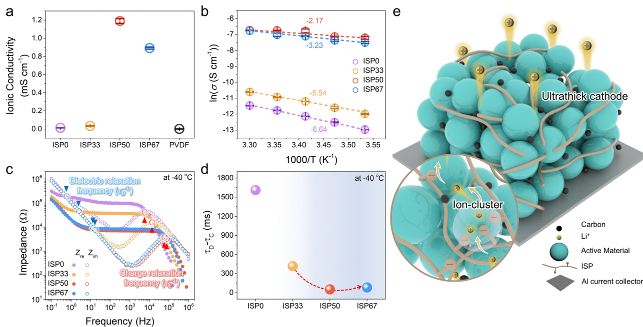
Fig. 2 (a) Ionic conductivity of the ISP series and PVDF. (b) Ionic conductivity depending on the temperature of the ISP series. (c) Real and imaginary impedance depending on the frequencies, and the (d) ion migration relaxation time of the ISP series at -40 °C. (e) Schematic diagram of ion clusters in the ultrathick cathode.
