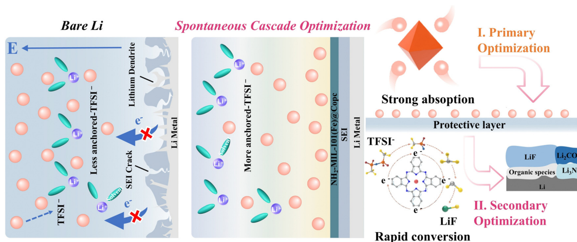
Fig. 1 Schematic diagram of the principle of the modification layer \text{NH}_2\text{-MIL-101(Fe)@Copc} .
