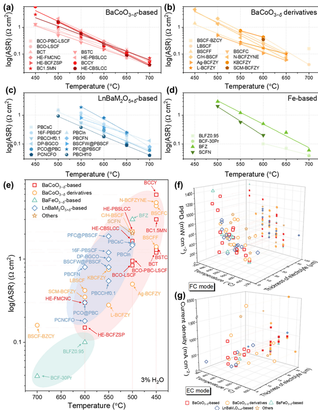
Fig. 16 Comparison of ASR in symmetrical cell configuration of advanced air electrodes for P-SOCs at 3% H 2 O: (a) BaCoO 3-δ -based perovskites, (b) BaCoO 3-δ -derived perovskites, (c) LnBaM 2 O 6+δ -based perovskites, and (d) Fe-based perovskites. Summary of electrochemical properties of advanced perovskite air electrode materials (detailed data summarized in Table 1): (e) ASR of lowest working temperature in symmetrical cells configuration, (f) PPDs in fuel cell (FC) mode, and (g) current densities in electrolysis cell (EC) mode.
