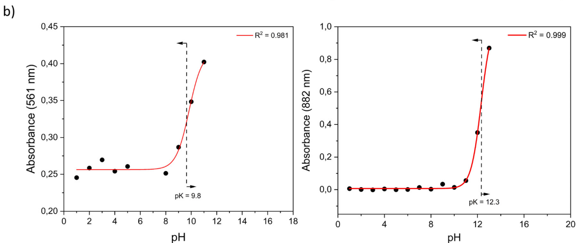
Fig. 5 (A) Proposed representative scheme for the nucleophilic attack reaction of the compound [\{\text{RuNO}\}^6\text{Ru}^{\text{III}}\text{Ru}^{\text{III}}\text{O}(\text{CH}_3\text{COO})_6(\text{py})_2]^+ by hydroxyl ions in aqueous media. (B) Sigmoidal fit of the spectrophotometric monitoring data collected for complex 2 ( \lambda_{\text{max}} = 561 and 882 nm) in aqueous solutions at different values of pH.
