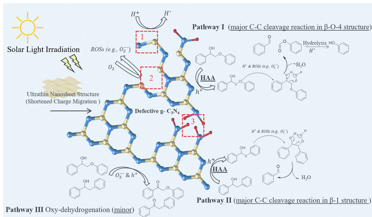
Scheme 13 Proposed mechanism of multi-defective \text{g-C}_3\text{N}_4 photocatalysed cleavage of C–C bonds in \beta\text{-O-4} and \beta\text{-1} structures; the marked area 1, 2 and 3 represent the -\text{C}\equiv\text{N} , N vacancy and C vacancy, respectively (this scheme has been reproduced from ref. 90 with permission from Elsevier, copyright 2024).
