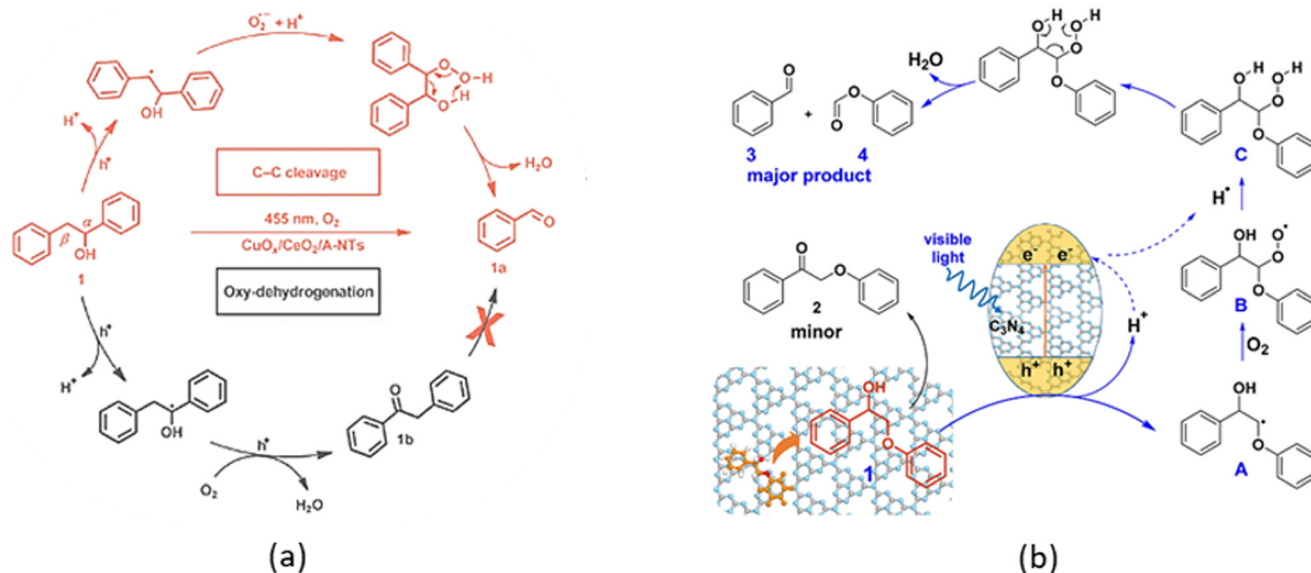
Scheme 12 The proposed reaction mechanism for photocatalytic cleavage of the \text{C}_\alpha - \text{C}_\beta bond in the (a) \beta -1 lignin model compounds over the \text{CuO}_x/\text{CeO}_2/\text{TiO}_2 catalyst and (b) in the \beta -O-4 lignin model compounds over mpg- \text{C}_3\text{N}_4 catalysts (this scheme is reproduced from ref. 66 and 88 with permission from American Chemical Society, copyright 2017 & copyright 2018).
