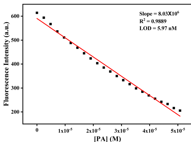
Fig. 12 The linear calibration plot of [PA] vs. photoluminescence to estimate the LOD and LOQ values for the recognition of PA ions utilizing MBB microparticles.
