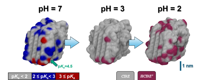
Fig. 5 Snapshots of the CBZ crystallite as obtained from MD simulations in aqueous solution (solvent not shown) at various \text{pH} values. Left: CBZ crystal at \text{pH} = 7 . A color code is used to indicate local differences in proton affinity – quantified in terms of the predicted \text{pK}_a value of the corresponding acid. While one particularly exposed CBZ experiences protonation at \text{pH} < 4.5 , we find 9 candidates for CBZ protonation at \text{pH} = 3 , as compared to 71 possible protonation sites at \text{pH} = 2 , respectively. Center & right: CBZ/CBZH core/shell nanocrystal models as obtained at \text{pH} = 3 and 2, respectively. Note that no dissociation is observed thus leading to +9 and +71 charged crystallite models of +0.005 and +0.03 \text{ C m}^{-2} surface charge density, respectively.
