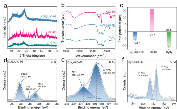
Fig. 1 (a) XRD patterns, (b) FT-IR spectra, and (c) zeta potential values of C_3N_4 /UiO-66, UiO-66 and C_3N_4 . (d) C 1s, (e) N 1s and (f) Zr 3d regions of the XPS spectrum of C_3N_4 /UiO-66.
