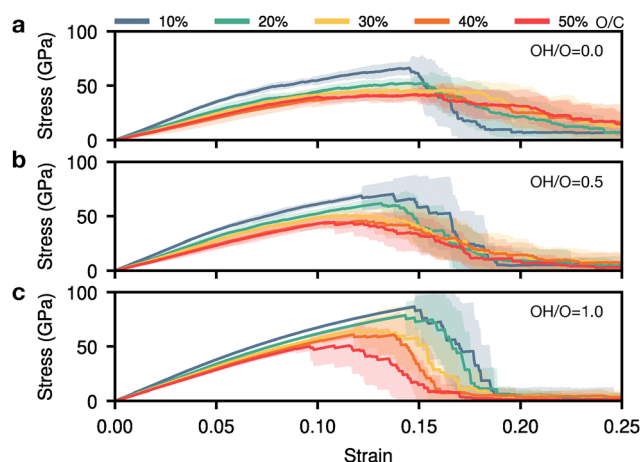
Fig. 2 Mechanical behaviour of GO and its dependence on the oxygen content. We show stress-strain curves for 20 GO sheets of ~200 atoms each, at varying O/C ratio (indicated by colour-coding). The shaded areas indicate one standard deviation. We characterise sheets that have been functionalised: (a) fully with epoxide groups; (b) with half epoxide, half hydroxyl groups; and (c) fully with hydroxyl groups.
