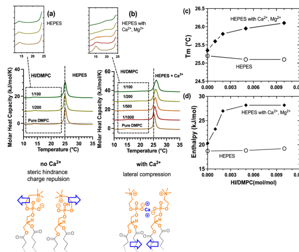
Fig. 5 DSC analysis of T_m and enthalpy changes upon addition of heparin (HI) to 1 \text{ mg mL}^{-1} DMPC LUVs in (a) HEPES buffer and (b) HEPES buffer plus \text{Ca}^{2+} , \text{Mg}^{2+} . Curves correspond to DMPC mixed with different amounts of HI. The pre-transition of DMPC is circled by the dashed rectangle and zoomed in the left top; corresponding main phase transition temperature (c) and enthalpy (d) of DMPC LUVs according to HI/DMPC ratio. The thermograms are from one experiment repeated once. Similar results with DPPC and DSPC in SI. Below thermograms (a) and (b) is represented the hypothesis for the impact of \text{Ca}^{2+} on PC organization: in the absence of \text{Ca}^{2+} , the positively charged choline interacts with the negative phosphate moiety of the polar head, which would create steric hindrance or charge repulsion between the polar head groups of adjacent phospholipids; in the presence of \text{Ca}^{2+} , the divalent ion bridging phosphate moieties would allow the choline headgroup to reorientate outside the bilayer and induce lateral compression between adjacent alkyl chains.
