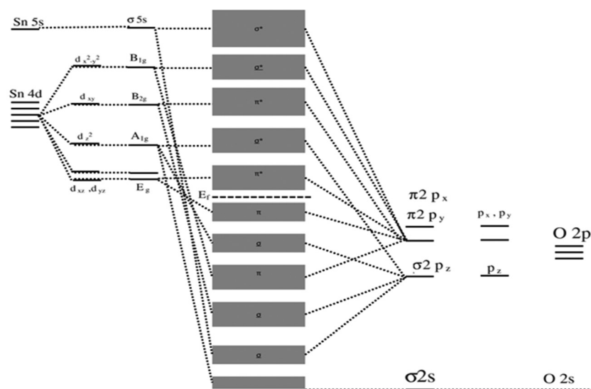
Fig. 8 Molecular-orbital bonding structure for tetragonal SnO 2 .
