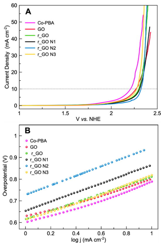
Fig. 7 Electrochemical experiments of Co-PBA and graphene-based materials performed in 0.5 \text{ mol L}^{-1} \text{ KNO}_3 at a scan rate of 5 \text{ mV s}^{-1} . (A) Linear sweep voltammetry (LSV) and (B) Tafel plot.
