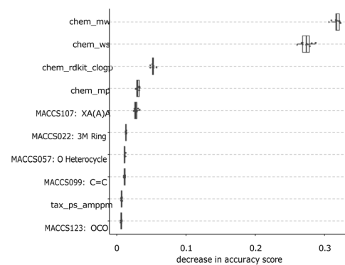
(b) Permutation-based feature importance.
