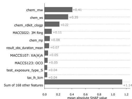
(c) Mean absolute SHAP values.
