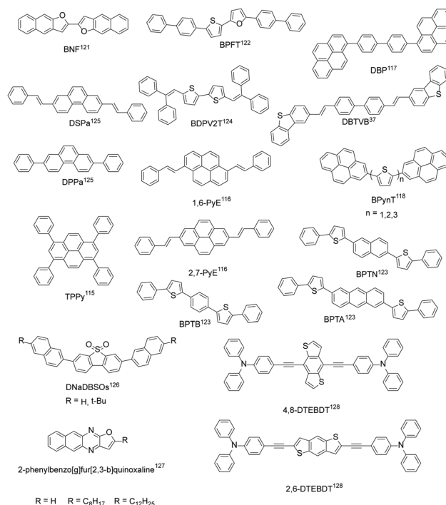
Fig. 7 Chemical structures of other organic fluorescent semiconductors reported.
