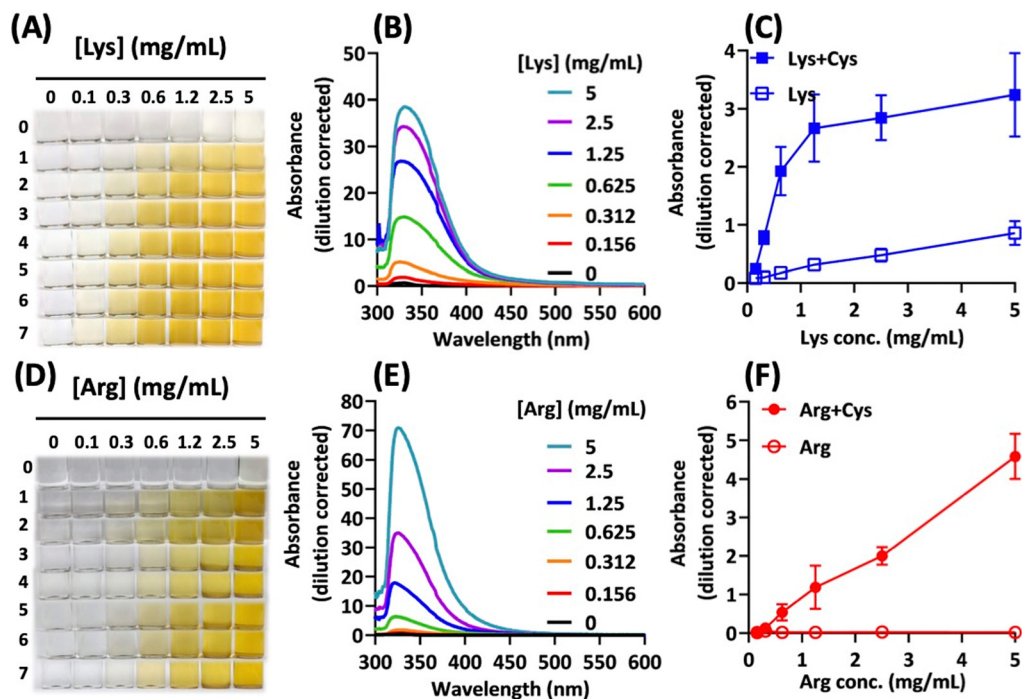
Fig. 1 Synergistic browning effect of lysine–cysteine and arginine–cysteine pairs. (A) Appearance of solution containing cysteine (1.25 mg mL -1 ) and increasing concentrations of lysine (0 to 5 mg mL -1 ) in DMSO/acetone (9/1), as shown from the initial time to day 7. (B) Dilution-adjusted UV-vis spectra of lysine–cysteine solutions at day 7. (C) Comparison of dilution-adjusted absorbance at 420 nm for lysine–cysteine combination solutions and lysine alone, at different lysine concentrations. (D)–(F) Counterparts of (A)–(C) for the arginine–cysteine pair.
