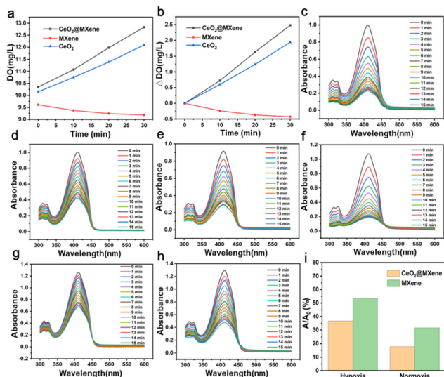
Fig. 3 Performance test of the \text{CeO}_2 @MXene material under irradiation light ( 808\text{ nm} , 1.0\text{ W cm}^{-2} ), and the test DPBF absorbance value at 410\text{ nm} wavelength: (a) Comparison of oxygen production of materials in the hydrogen peroxide solution ( 10\text{ mM} ). (b) Comparison of the oxygen productivity of materials in the hydrogen peroxide solution ( 10\text{ mM} ). (c) Singlet oxygen production from \text{CeO}_2 @MXene in hydrogen peroxide. (d) Singlet oxygen formation in water from \text{CeO}_2 @MXene. (e) Singlet oxygen production from MXene under normoxic conditions. (f) Singlet oxygen production from \text{CeO}_2 @MXene under normoxic conditions. (g) Singlet oxygen production from MXene under hypoxic conditions. (h) Singlet oxygen production from \text{CeO}_2 @MXene under hypoxic conditions. (i) Comparison of singlet oxygen production between \text{CeO}_2 @MXene and MXene under normoxic and hypoxic conditions.
