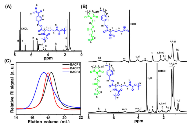
Fig. 1 (A) 1 H NMR spectrum of M2 . (B) 1 H NMR spectra of the protected polymer ( BACP3 ) in DMSO- d 6 and deprotected polymer ( ACPy3 ) in D 2 O. (C) SEC RI traces of BACP1 – BACP3 in DMF.
