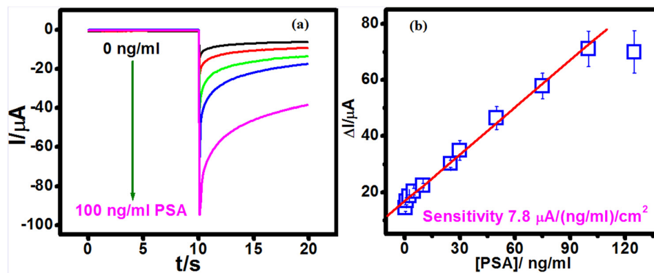
Fig. 6 (a) Amperometric curves of \text{OCD}@^{\text{PSA}}\text{Ab}_2 detection probe-based PSA biosensor in the presence of 3 mM HQ and 4.5 mM \text{H}_2\text{O}_2 at different concentrations of PSA and (b) the calibration plot for the \text{OCD}@^{\text{PSA}}\text{Ab}_{\text{HRP}} -based PSA biosensor.
