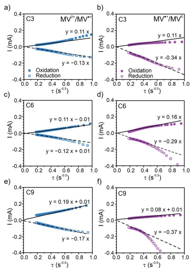
Fig. 4 Chronoamperometry (CA) Cottrell plots for the two redox couples of the three polypeptides. (a), (c), and (e) CA response for the MV^{2+}/MV^{+} redox couple. (b), (d), and (f) CA response for the MV^{+}/MV^0 redox couple. Viologen polypeptides coated on ITO glass were used as the working electrodes in a three-electrode beaker cell configuration. The supporting electrolyte was 0.5 M LiCl in GBL. Lithium metal was used as counter and reference electrodes. The Cottrell plots for PV are found in Fig. S25.†
