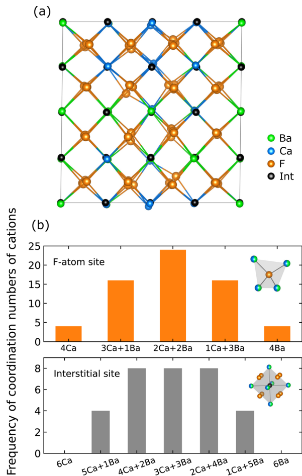
Fig. 2 (a) Relaxed SQS structure in the 2 \times 2 \times 2 conventional supercell of Ba 0.5 Ca 0.5 F 2 and (b) histogram of the combination of coordinating cations around the F-atom sites (8c) and interstitial sites (4b) in the fluorite supercell.
