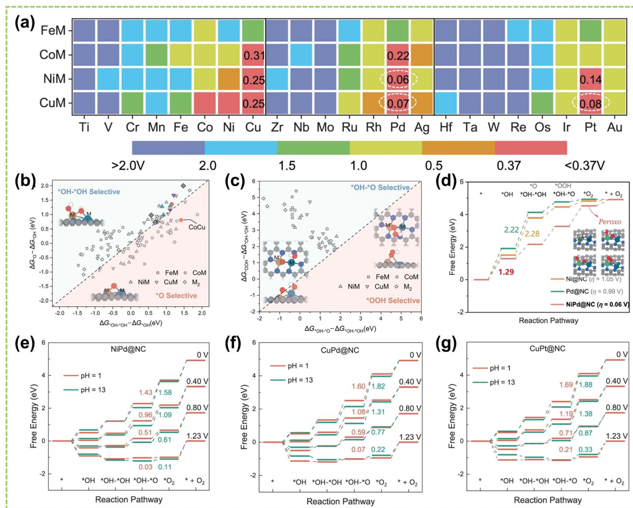
Fig. 19 The OER performance of DACs in all pH conditions. (a) Activity map. The computed overpotential of the FeM, CoM, NiM, and CuM dimers on M'@NC. (b) \Delta G of ^*OH toward ^*OH-^*OH versus ^*OH \rightarrow ^*O + H^+ + e^- . Data points screened for high-performance homo- and hetero-nuclear catalysts are colored. (c) \Delta G of ^*OH-^*OH \rightarrow ^*OH-^*O + H^+ + e^- versus ^*OH-^*OH \rightarrow ^*OOH + H^+ + e^- . Insets: the schematic configuration of the different intermediates adsorbed on M'@NC. The white, red, gray, and blue spheres in the atomic models represent H, O, C, and N atoms, respectively. (d) Free energy diagrams of NiPd@NC and the respective corresponding SACs for OER. Inset: the optimized configurations of oxygenated intermediates represented as NiPd@NC. Free energy diagrams of (e) NiPd@NC, (f) CuPd@NC, and (g) CuPt@NC at different potentials with pH = 1 and 13 and the corresponding \Delta G_{^*OH-^*O \rightarrow ^*O_2} are labeled 89 (reproduced with permission from ref. 89 copyright 2023, Springer Nature).
