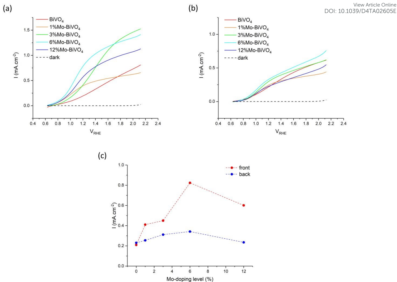
Figure 6: Current voltage (JV) curves for BiVO 4 and all Mo-doped BiVO 4 samples measured with (a) front irradiation and (b) back irradiation. (c) The photocurrent densities observed at 1.23 V RHE for both front and back irradiation as a function of Mo precursor doping level (%) of BiVO 4 and all Mo-doped BiVO 4 samples. Samples were measured in 0.1 M phosphate buffer (pH = 7) using 400 nm light (~8.5 mW.cm -2 ).
