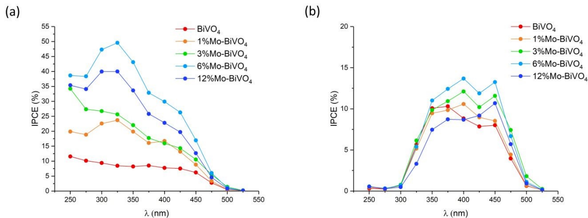
Figure 7: Incident photon to current efficiency (IPCE) curves for \text{BiVO}_4 and all Mo-doped \text{BiVO}_4 samples measured with (a) front irradiation and (b) back irradiation. Samples were measured in 0.1 M phosphate buffer (pH = 7) at 1.23 V_{\text{RHE}} .
