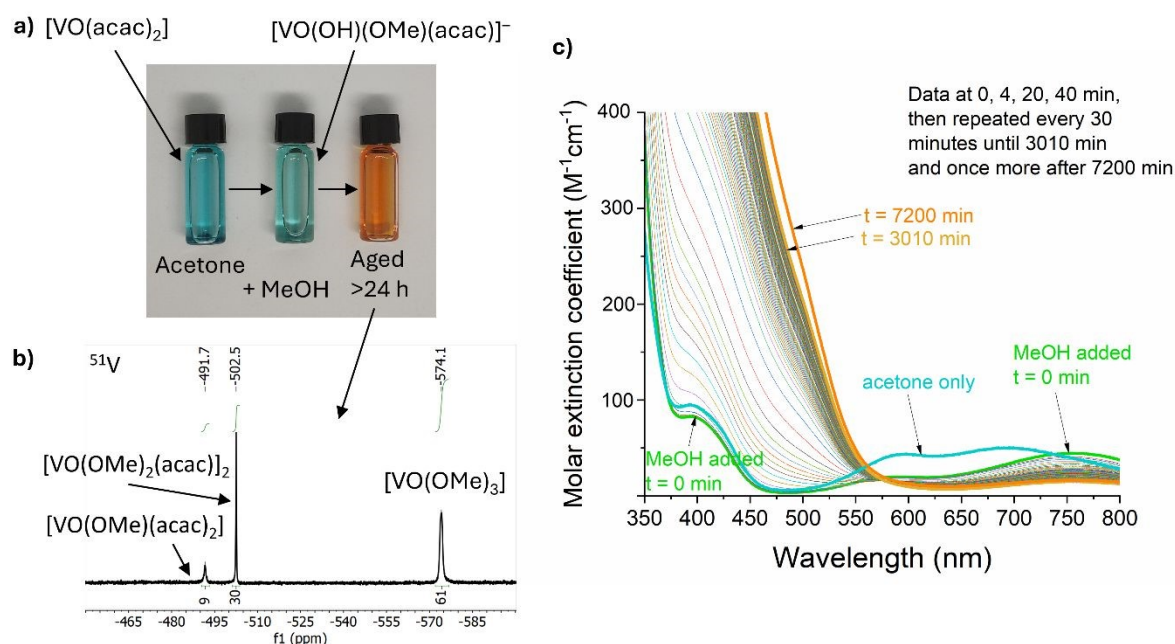
Figure 1: (a) Photos (left to right) of \text{VO}(\text{acac})_2 dissolved in acetone, acetone/MeOH, and then after ageing under air. (b) ^{51}\text{V} NMR spectrum of a 5 mM solution of \text{VO}(\text{acac})_2 + \text{BiPh}_3 in deuterated acetone/MeOH (3:1) after oxidation for 30 h under air. (c) Visible absorption spectra of a 5mM solution of \text{VO}(\text{acac})_2 in acetone (bold blue line) and 5mM solution of \text{VO}(\text{acac})_2 in acetone/MeOH (3:1) over time (bold green line, t = 0 min; bold gold line, t = 3010 min; bold orange line, t = 7200 min). \text{BiPh}_3 was added at the end of the experiment but has no effect on the absorption spectrum.
