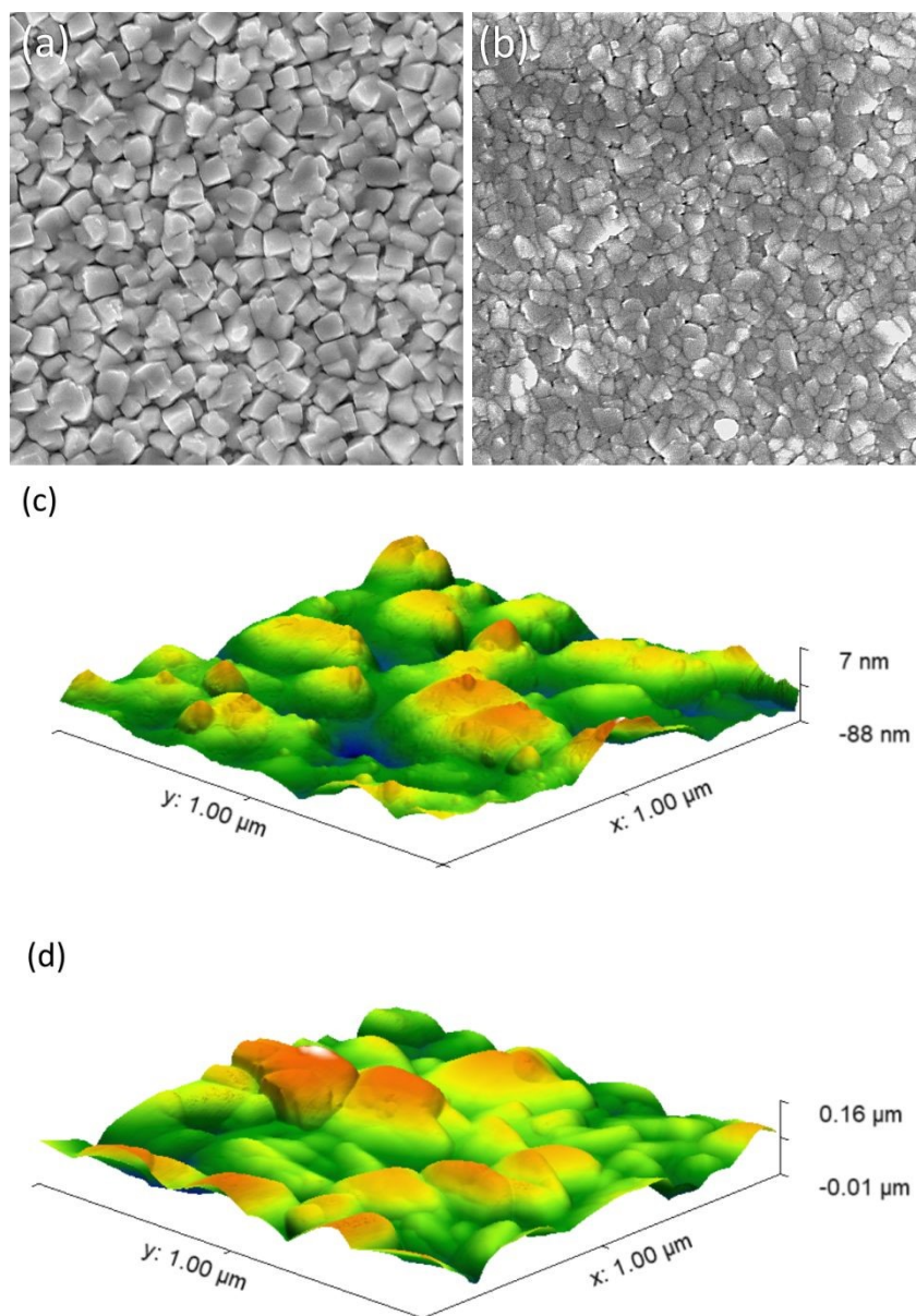
Figure 4: SEM images of (a) \text{BiVO}_4 and (b) 6%Mo- \text{BiVO}_4 taken at 50k magnification [the width of each image represents a distance of 3.8 \mu\text{m} ]. AFM images, of (c) \text{BiVO}_4 and (dc) 6%Mo- \text{BiVO}_4 measured over a 1 \mu\text{m} x 1 \mu\text{m} square area.
