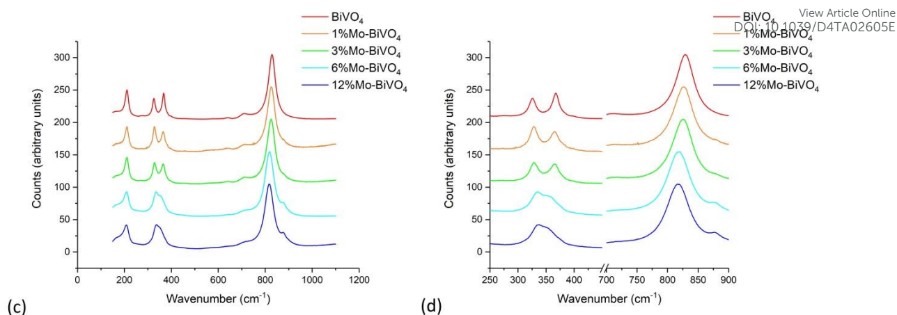
Figure 2: (a) XRD patterns, (b) close-up view of select peaks in XRD patterns, (c) Raman spectra and (d) close-up view of select peaks in Raman patterns of \text{BiVO}_4 and all Mo-doped \text{BiVO}_4 samples.
