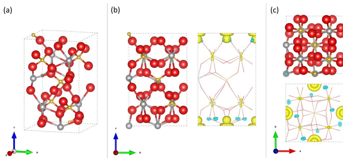
Figure 10: Calculated structure for 12.5 at.% Mo doping of a V site in tetragonal scheelite \text{BiVO}_4 for a single unit cell showing atomic positions and spin density [Bi = silver, V = gold, O = red, Mo = light blue; ionic radii proportions scaled down for visibility]. (a) angled view, (b) a-axis view and (c) c-axis view.
