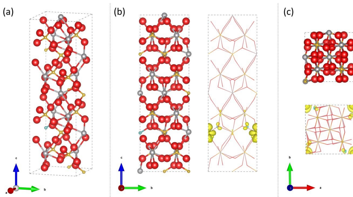
Figure 9: Calculated structure for 6.25 at.% Mo doping of a V site in t\text{-BiVO}_4 for a 2 \times 1 \times 1 supercell showing atomic positions and spin density [Bi = silver, V = gold, O = red, Mo = light blue; ionic radii proportions scaled down for visibility]. (a) angled view, (b) a -axis view and (c) c -axis view.
