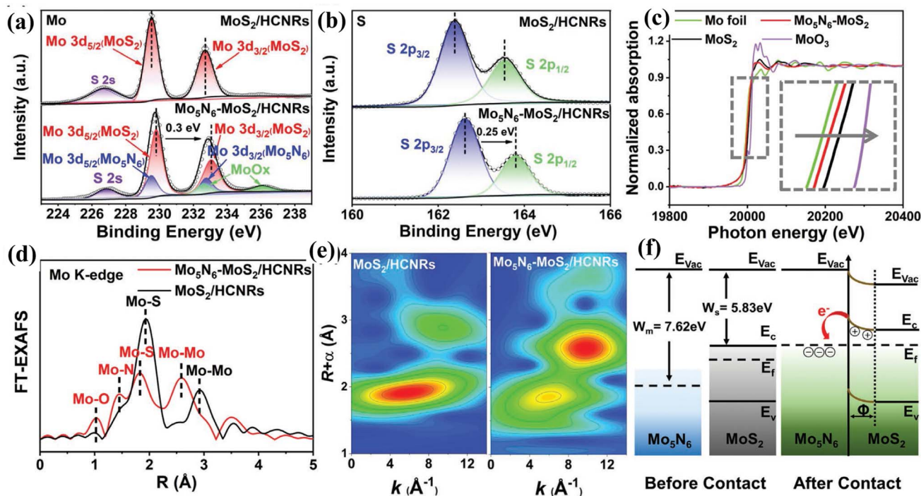
Fig. 6 High-resolution XPS spectra of (a) Mo 3d and (b) S 2p obtained from Mo 5 N 6 -MoS 2 /HCNRs in comparison with 2H-MoS 2 /HCNRs; (c) Mo K-edge XANES spectrum of Mo 5 N 6 -MoS 2 /HCNR in comparison with Mo foil, MoO 3 , and 2H-MoS 2 /HCNRs; (d) FT-EXAFS curves and (e) WT-EXAFS of Mo 5 N 6 -MoS 2 /HCNRs in comparison with 2H-MoS 2 /HCNRs, disclosing the generation of the N-Mo-S triatomic interface and in-plane electronic coupling between MoS 2 and Mo 5 N 6 ; (f) schematic illustration depicts the energy band of the Schottky-type Mo 5 N 6 -MoS 2 heterojunction, where the electron is transferred from 2H-MoS 2 to Mo 5 N 6 due to the metallic Mo 5 N 6 /semiconducting MoS 2 heterojunction ( E_{\text{vac}} = vacuum energy, E_{\text{g}} = energy gap, E_{\text{c}} = conduction band, E_{\text{f}} = Fermi level, E_{\text{v}} = valence band, \Phi = depletion region, and W = work function) (reproduced with permission from ref. 108 Copyright 2022, Wiley-VCH GmbH).
