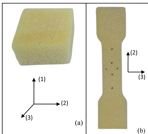
Fig. 2 Compressive (a) and tensile (b) foam samples.
