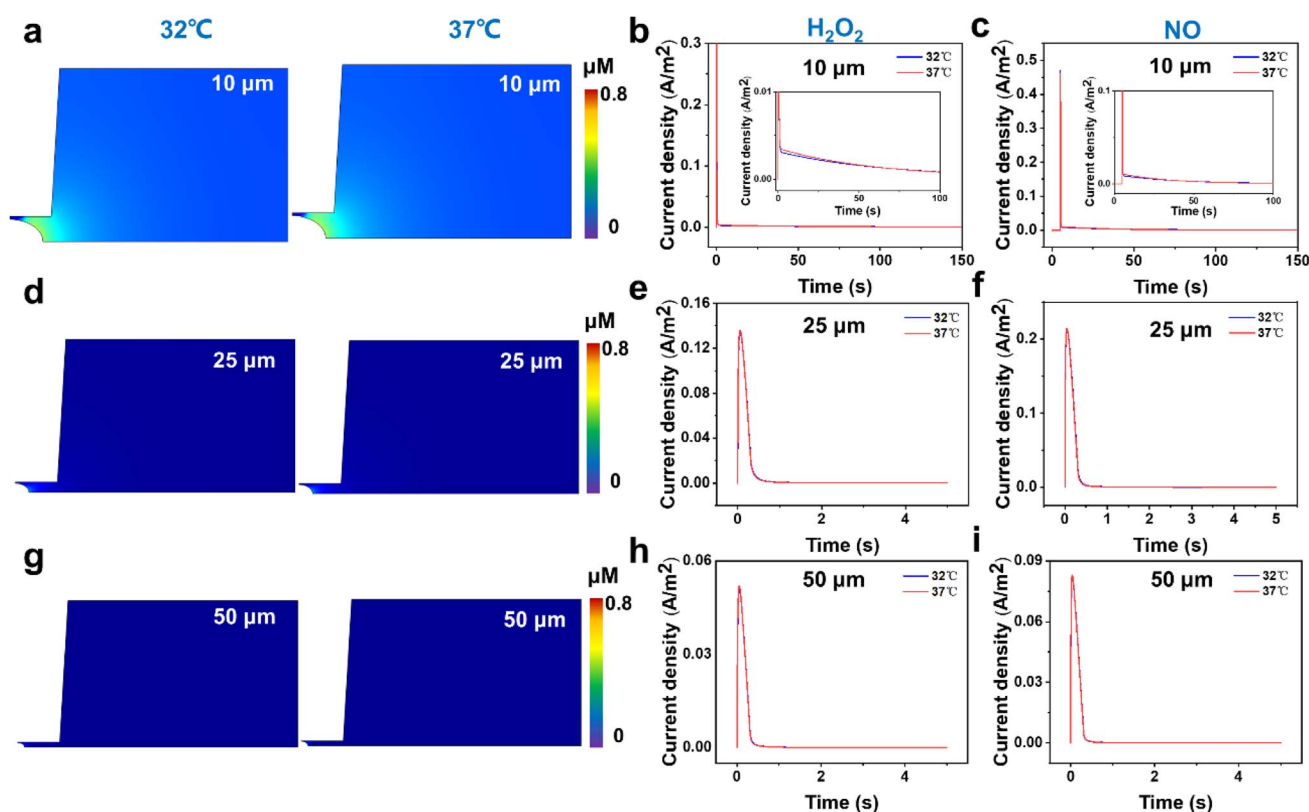
Fig. 3 FEM stimulations of (a, d and g) concentration maps of \text{H}_2\text{O}_2 effluxes and (b, c, e, f, h and i) amperometric traces of \text{H}_2\text{O}_2 and NO effluxes released from the cell membrane at 32 °C and 37 °C using (a–c) 10, (d–f) 25 and (g–i) 50 \mu\text{m} -in-diameter microdisk electrodes as the SECM probes. The insets of (b) and (c) are the magnified images of each amperometric trace in the first 100 s in the current density range of 0–0.1 \text{A m}^{-2} .
