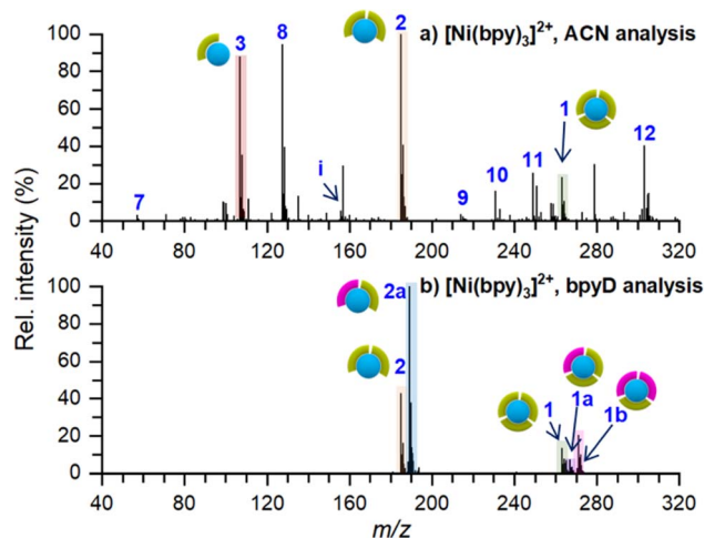
Fig. 2 Ex situ nano-DESI MS of the deposition spots of [Ni(bpy) 3 ] 2+ analyzed with (a) ACN and (b) 3 μM bpyD in ACN as the nano-DESI solvent. Ion assignments are listed in Table 1. The pictograms symbolize the number of ligands coordinated to Ni. Green and pink symbols represent bpy and bpyD, respectively. Peaks originating from the solvent are not marked in the spectra for simplicity.
