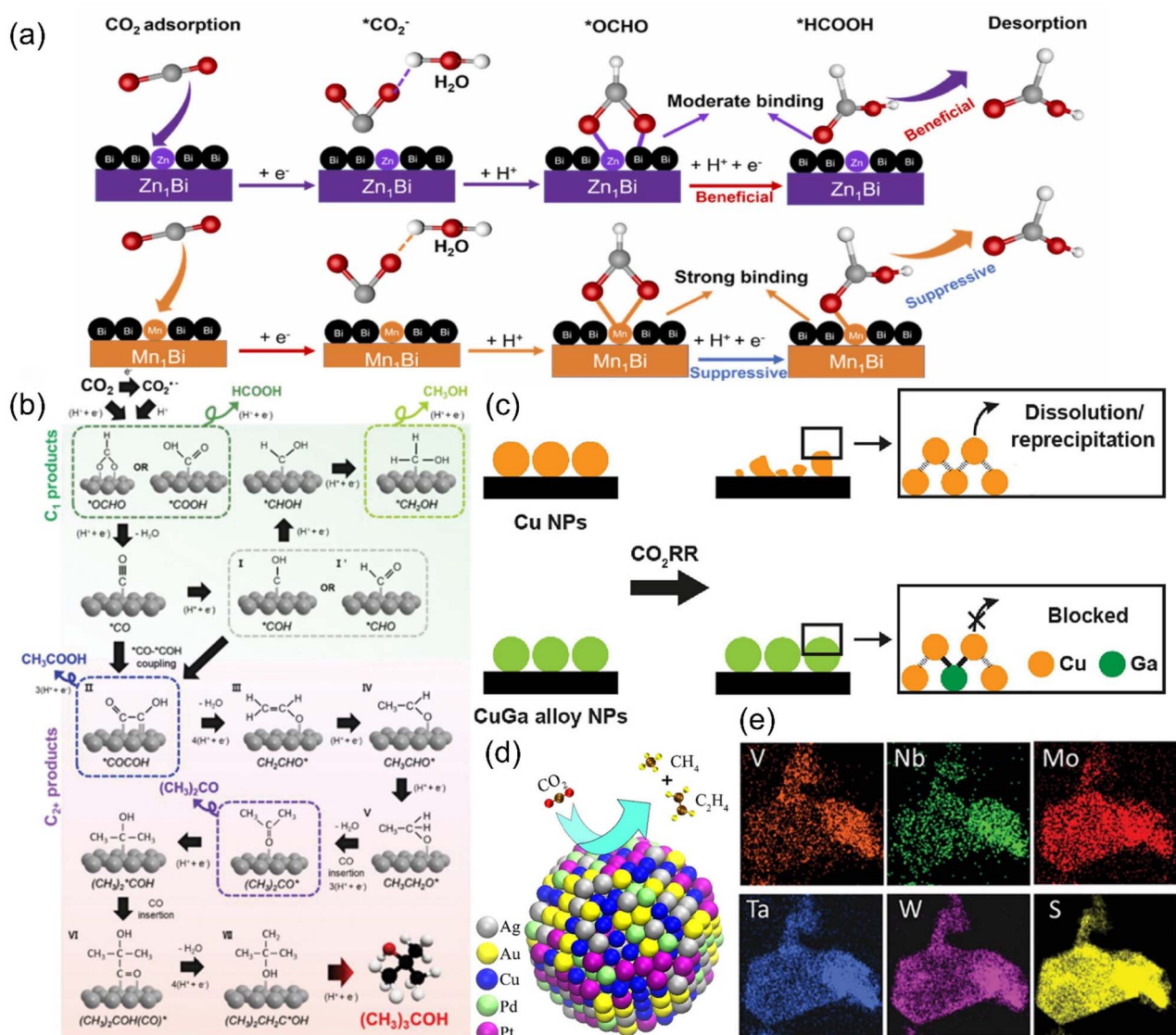
Fig. 21 (a) A proposed reaction mechanism for CO 2 R to formate on SAA-Zn 1 Bi and SAA-Mn 1 Bi. (b) A probable mechanism for CO 2 R to (CH 3 ) 3 COH. (c) Illustration of the CO 2 RR stabilization mechanism on CuGa alloy NPs. (d) Schematic of the catalysis reaction on AuAgPtPdCu. (e) EDS maps of (MoWVNbTa) 2 S 2 . (a) Reproduced with permission. 233 Copyright 2023, Elsevier Ltd. (b) Reproduced with permission. 236 Copyright 2023, Wiley-VCH GmbH. (c) Reproduced with permission. 237 Copyright 2023, American Chemical Society. (d) Reproduced with permission. 240 Copyright 2020, American Chemical Society. (e) Reproduced with permission. 241 Copyright 2021, Wiley-VCH GmbH.
