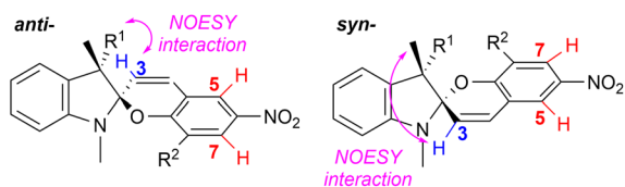
Fig. 4 Signal assignment of the syn - and anti -epimers based on NMR NOESY experiments; the syn : anti ratios were calculated using signals of the H-3 protons or H-5/H-7 protons from 1 H NMR spectra.
