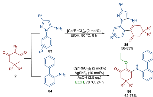
Scheme 43 Rh-catalyzed annulation of 1-aryl-1H-pyrazol-5-amine with cyclic 2-diazo-1,3-diketones.
