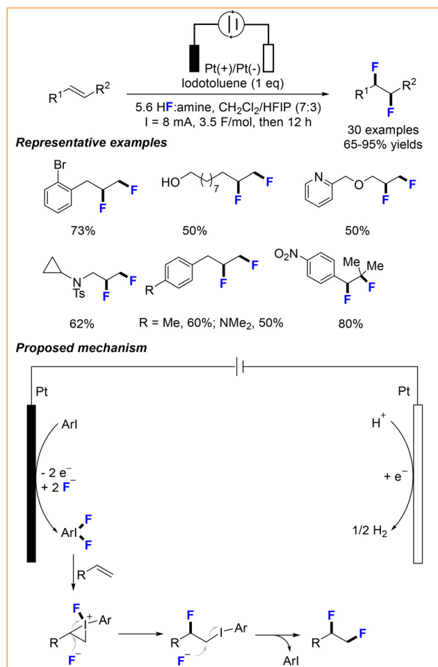
Scheme 3 Electrochemical vicinal difluorination of alkenes. 17
