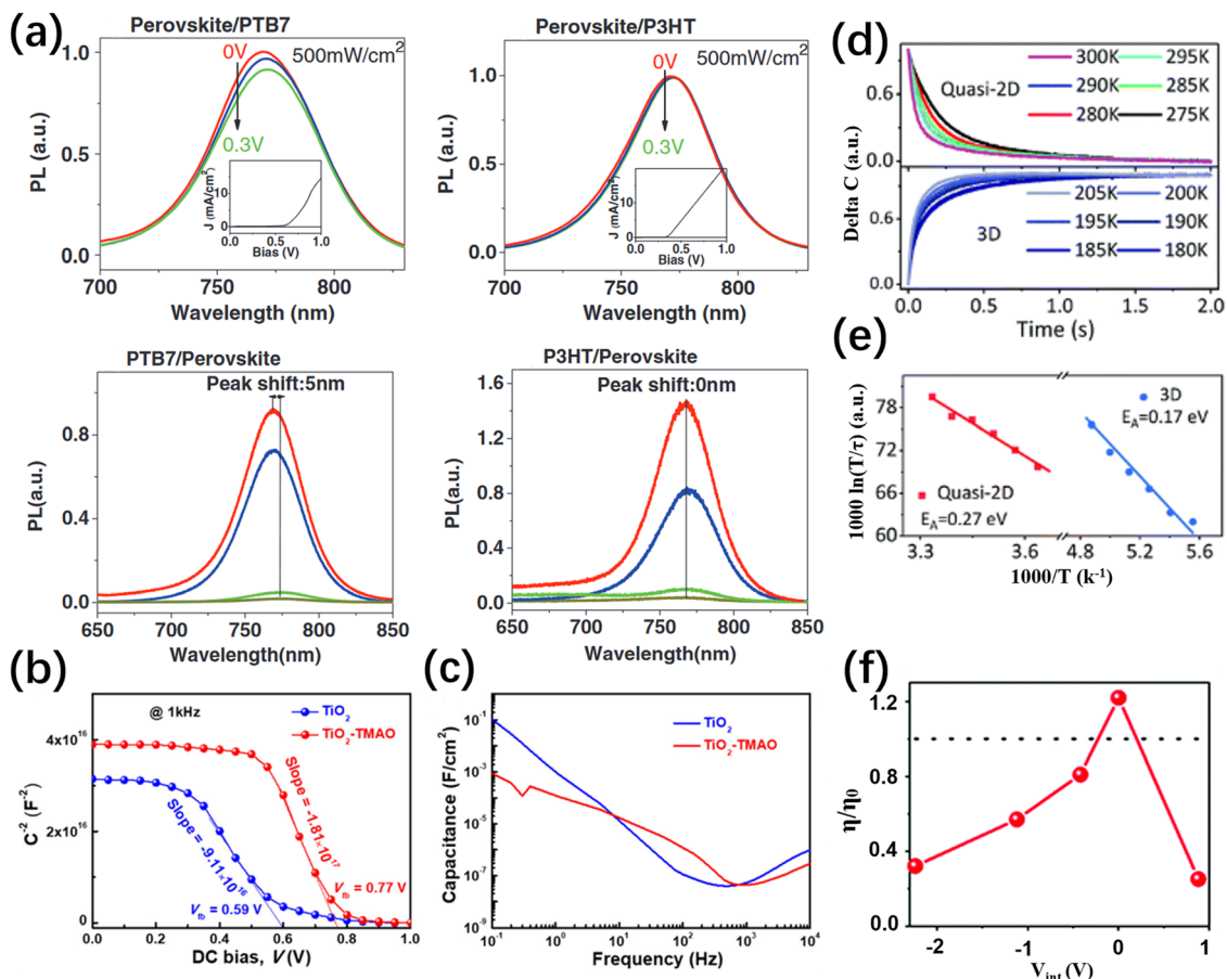
Fig. 21 (a) Electric field-induced photoluminescence spectroscopy. 170 Copyright 2017, Wiley. (b) Mott-Schottky analysis. (c) C - F plots. (d) Capacitance transients from anion migration (drift). 171 Copyright 2019, ACS. (e) Arrhenius fitting results of anion migration. (f) The function of the thermal-electrical poling voltage. 173 Copyright 2022, RSC.
