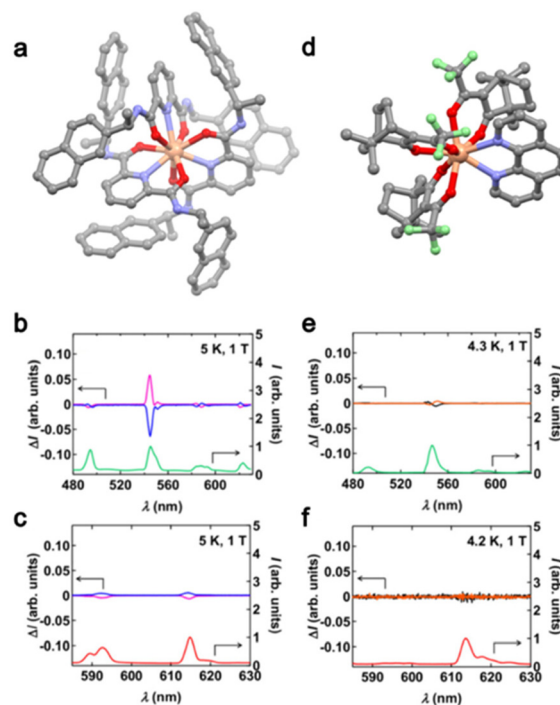
Fig. 1 (a) Molecular structure of (S,S)\mathbf{2-Tb} . Grey, C; red, O; blue, N and salmon, Tb. H atoms and \text{CF}_3\text{SO}_3^- anions are omitted for clarity. (b) Average luminescence spectrum of (S,S)\mathbf{2-Tb} (green line) and MChD spectra of (S,S)\mathbf{2-Tb} (pink line) and (R,R)\mathbf{2-Tb} (blue line). (c) Average luminescence spectrum of (S,S)\mathbf{2-Eu} (red line) and MChD spectra of (S,S)\mathbf{2-Eu} (pink line) and (R,R)\mathbf{2-Eu} (blue line). (d) Molecular structure of (d)\mathbf{3-Tb} . Grey, C; red, O; blue, N; green, F and salmon, Tb. H atoms are omitted for clarity. (e) Average luminescence spectrum of (d)\mathbf{3-Tb} (green line) and MChD spectra of (d)\mathbf{3-Tb} (black line) and (l)\mathbf{3-Tb} (orange line). (f) Average luminescence spectrum of (d)\mathbf{3-Eu} (red line) and MChD spectra of (d)\mathbf{3-Eu} (black line) and (l)\mathbf{3-Eu} (orange line). Adapted with permission from ref. 12. Copyright 2019, American Physical Society.
