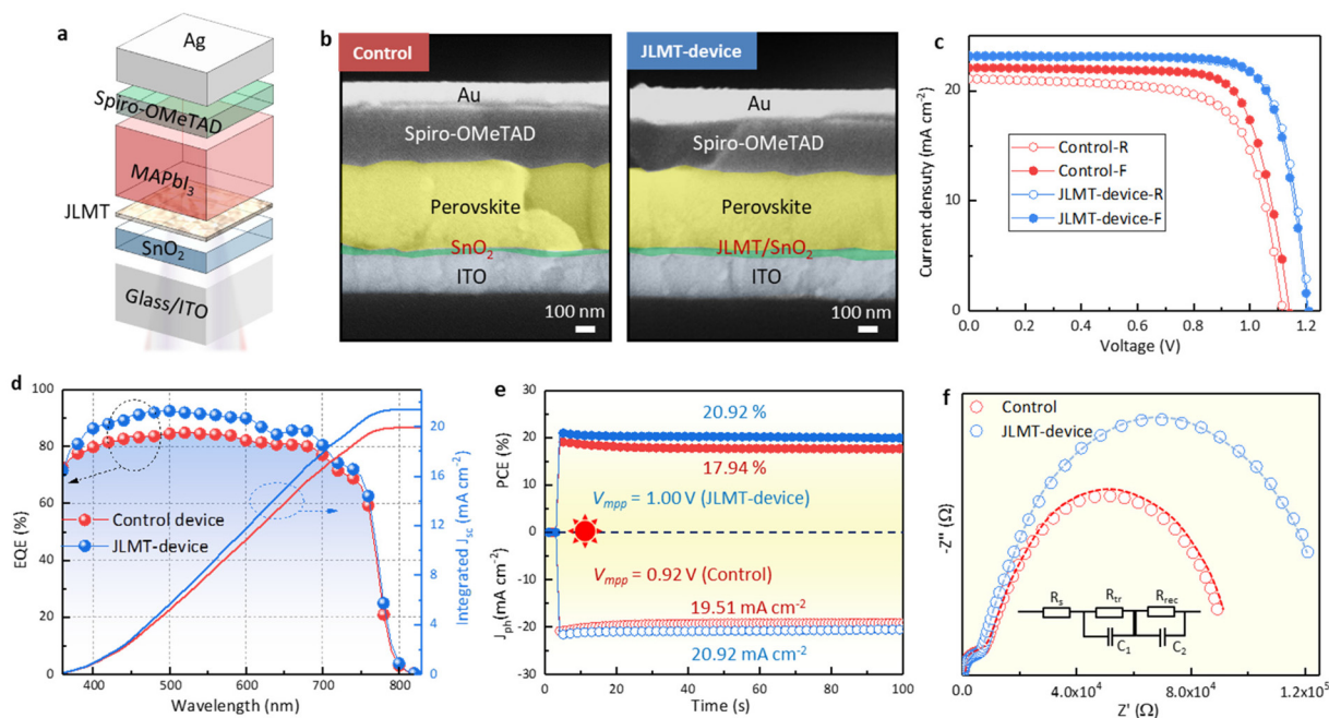
Fig. 7 Device performance (a) Whole device structure. (b) Cross-sectional SEM images of the control and JLMT devices. (c) Illuminated J-V curves of the control and JLMT devices. (d) EQE spectra and integrated photocurrent of the control and JLMT devices. (e) PCE and output current density measured at the V_{\text{mpp}} of the control and JLMT devices. (f) Nyquist plots of the control and JLMT devices. The inset shows the equivalent circuit model.
