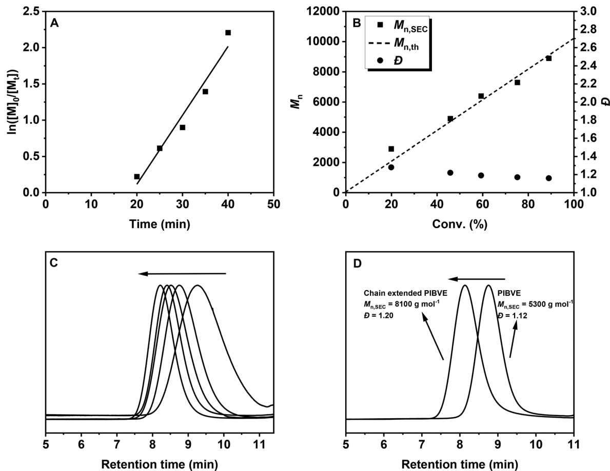
Fig. 2 Polymerization of IBVE with [IBVE] 0 /[DTCB] 0 /[DPI] 0 /[Ir(ppy) 3 ] 0 = 100/1/0.01/0.0001 under a 450 nm blue LED at -30 °C in toluene and DCM (v/v = 9:1), V IBVE = 1 mL, V solvent = 1 mL. (A) ln([M] 0 /[M] t ) versus time. (B) Molecular weight ( M n ) and molecular weight distribution ( D ) versus monomer conversion; (C) SEC traces of the obtained PIBVE; (D) SEC traces of the PIBVE before and after chain extension.
