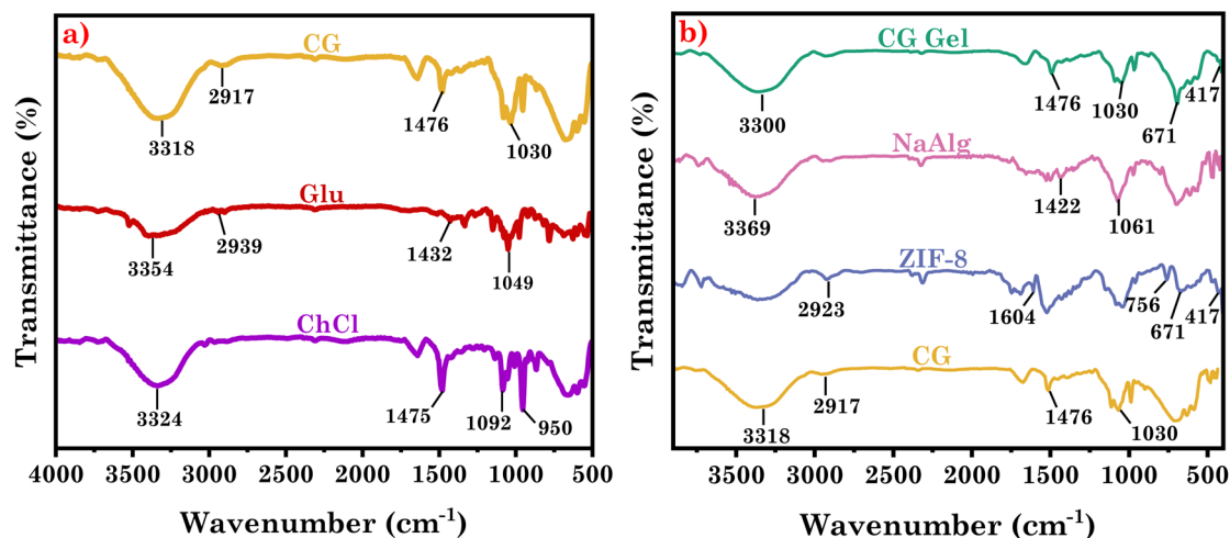
Fig. 1 FT-IR spectra of (a) ChCl, Glu and, CG; (b) CG, SA, ZIF-8, CG Gel.
