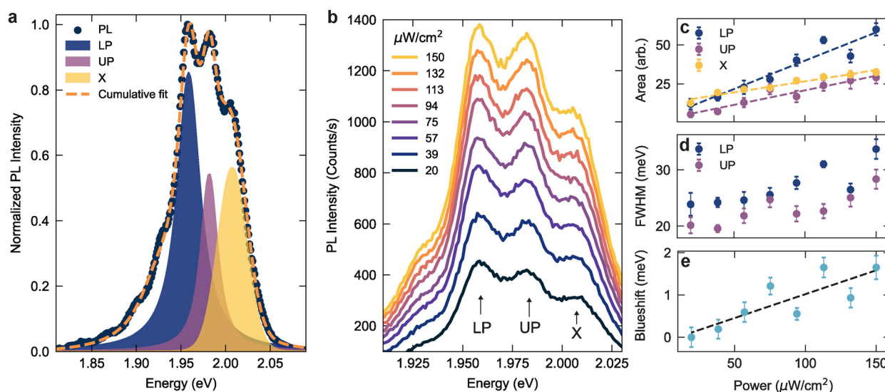
Fig. 4 (a) PL emission of monolayer \text{WS}_2 embedded in a hybrid nanocavity (GaP nanoantenna radius of 85 nm). The emission peaks are fitted with Voigt profiles. The uncoupled exciton (X) exhibits a Gaussian broadening, while the polariton branches are predominantly characterized by Lorentzian profiles. The dashed orange line is the cumulative fit. (b) Hybrid nanocavity-coupled \text{WS}_2 PL emission as a function of the excitation power. (c and d) Integrated peak area (c) and full width at half maximum (FWHM) (d) extracted from Voigt profile fits of the data in (b). (e) Blueshift of the PL dip, fitted with a Gaussian function. The dashed lines in (c and e) are linear fits to the respective data.
