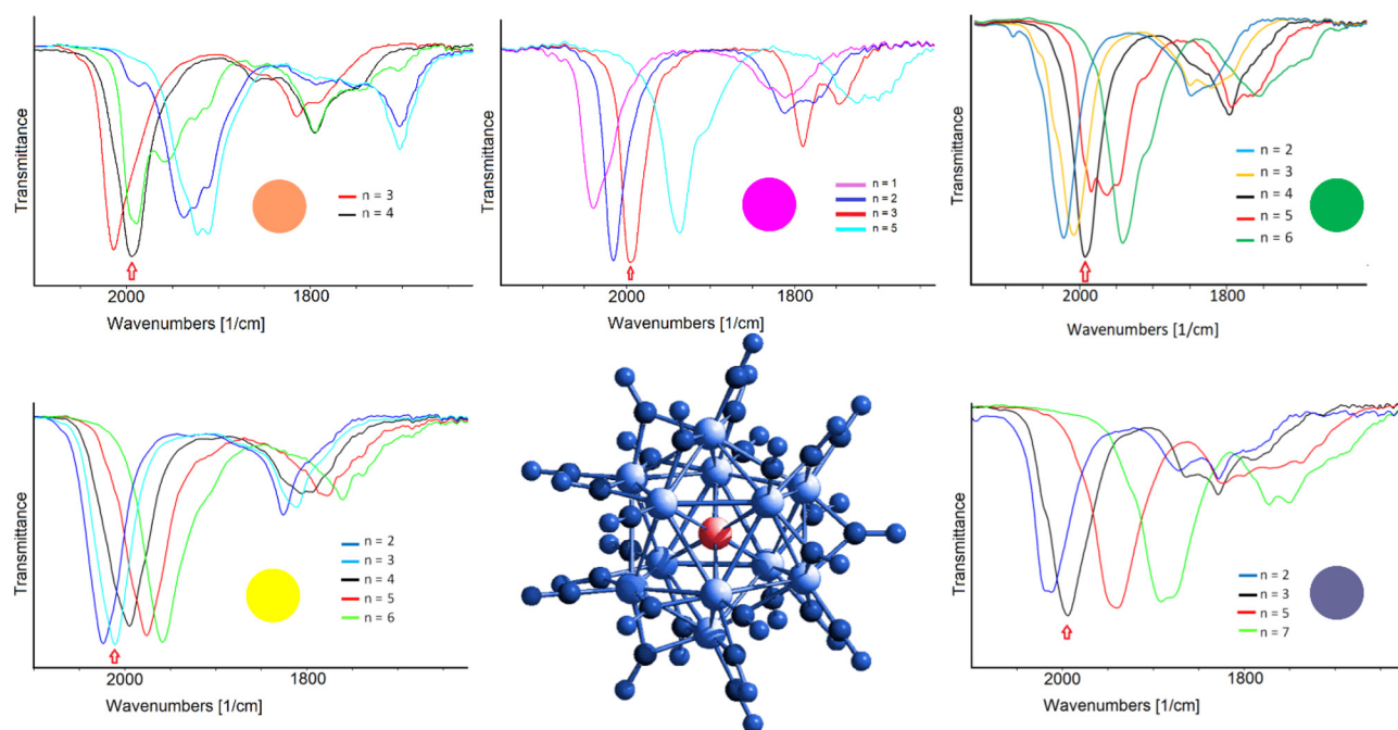
Fig. 8 Multivalence behaviour of the [\text{Rh}_{12}\text{E}(\text{CO})_{27/28}]^{n-} family of clusters ( n = 3 when \text{E} = \text{In}, \text{Sb}, \text{Bi} ; n = 4 when \text{E} = \text{Ge}, \text{Sn} ) as obtained by spectro-electrochemical experiments. 27
