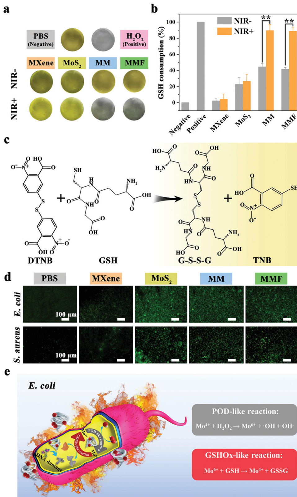
Fig. 7 GSH mechanism involved for evaluating the antibacterial effect of Ti 3 C 2 MXene/MoS 2 2D Bio-Heterojunctions. (a) Shows the changes in colour of GSH in different media. (b) Illustrates the percentage of GSH consumption with and without NIR irradiation applied to different materials. (c) Reaction of GSH with DTNB, giving GSSG and TNB as final products. (d) Images by fluorescence microscopy describing intracellular ROS production in different samples. (e) POD-like reaction compared to GSH-like reaction applied for E. coli . Reproduced with permission from ref. 66. Copyright 2021 Wiley-VCH GmbH.
