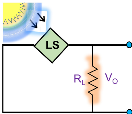
Fig. 1 Self-powered photodetector.
