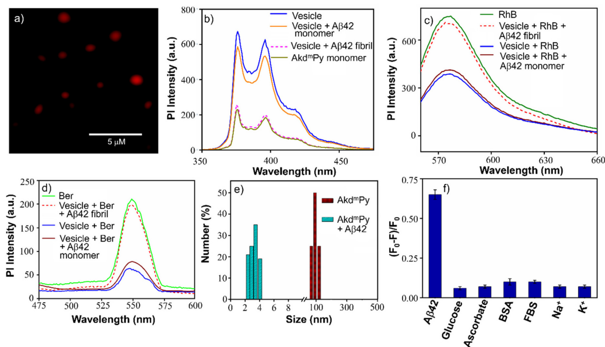
Fig. 4 (a) Fluorescence microscopy image of RhB entrapped within Akd m Py vesicles; (b) fluorescence emission spectra of Akd m Py monomer and molecular assembly of Akd m Py (40 \mu M) before and after treatment with A \beta 42 fibril and A \beta 42 monomer (10 \mu M); (c) fluorescence emission spectra of only RhB and RhB entrapped within Akd m Py vesicle before and after treatment with A \beta 42 fibril and A \beta 42 monomer (10 \mu M); (d) fluorescence emission spectra of only Ber and Ber entrapped within Akd m Py vesicle before and after treatment with A \beta 42 fibril and A \beta 42 monomer (10 \mu M); (e) size distribution of Akd m Py vesicles before (red) and after (cyan) treatment with A \beta 42 fibril; (f) relative change in fluorescence intensity of Akd m Py (40 \mu M) in the absence and presence of various biologically relevant species (10 \mu M). Percent errors are within \pm 5\% in triplicate experiments.
