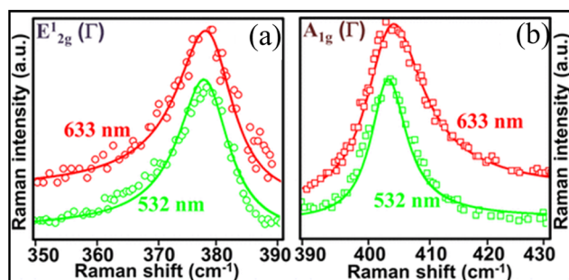
Fig. 9 Theoretical fitting (solid lines) of experimentally observed Raman spectra (discrete points) of MoS 2 nano-flakes corresponding to the E 2g mode (a) and A 1g mode (b) recorded using 633 and 532 nm laser excitation represented in red and green colours, respectively. Reproduced from ref. 36 with permission from [American Chemical Society], copyright [2022].
